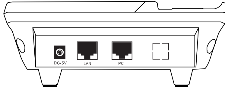
Figure 3-3 - Flexor 500 Rear Connectors and Connections
